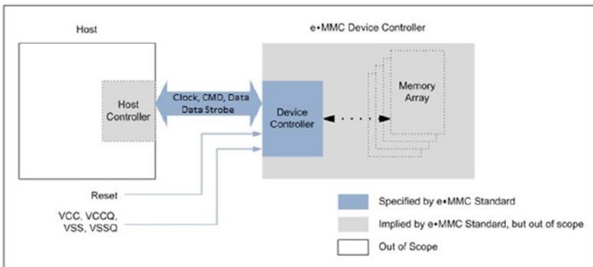
Figure 4-1 eMMC System Overview
