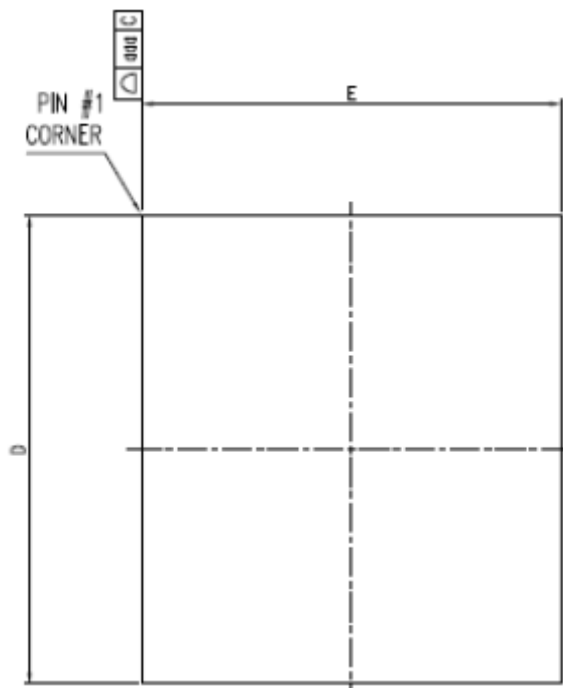
Figure 7-1 Top View
