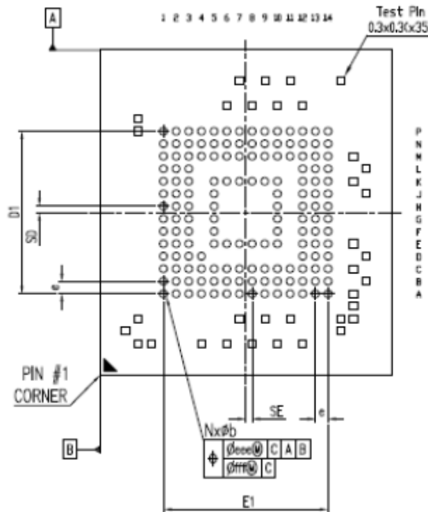
Figure 7-3 Bottom View
