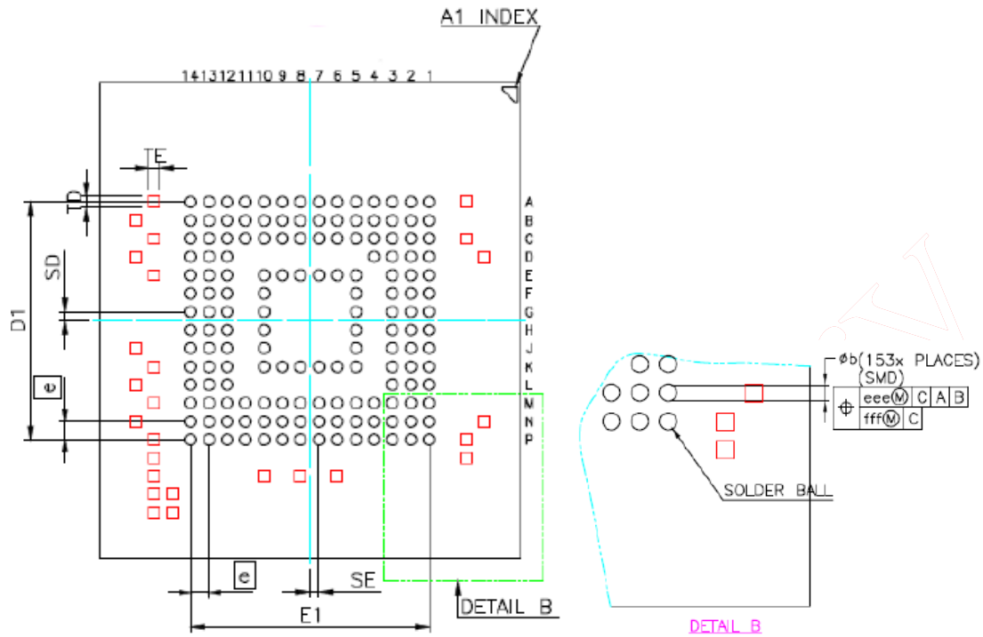
Figure 8-3 Bottom View
