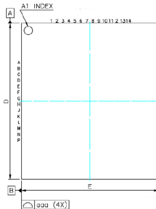
Figure 8-1 Top View
