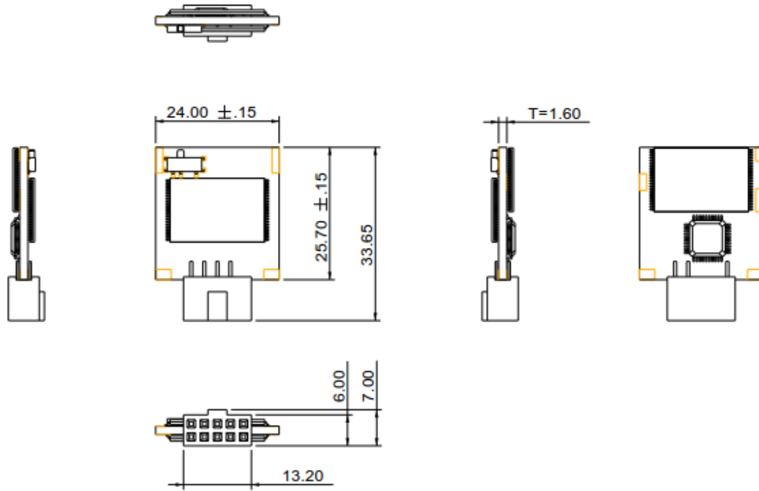
Figure 7-1 Physical Dimensions without Housing
