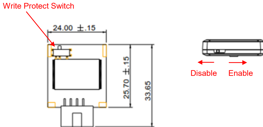
Figure 7-3 Write Protect Switch
