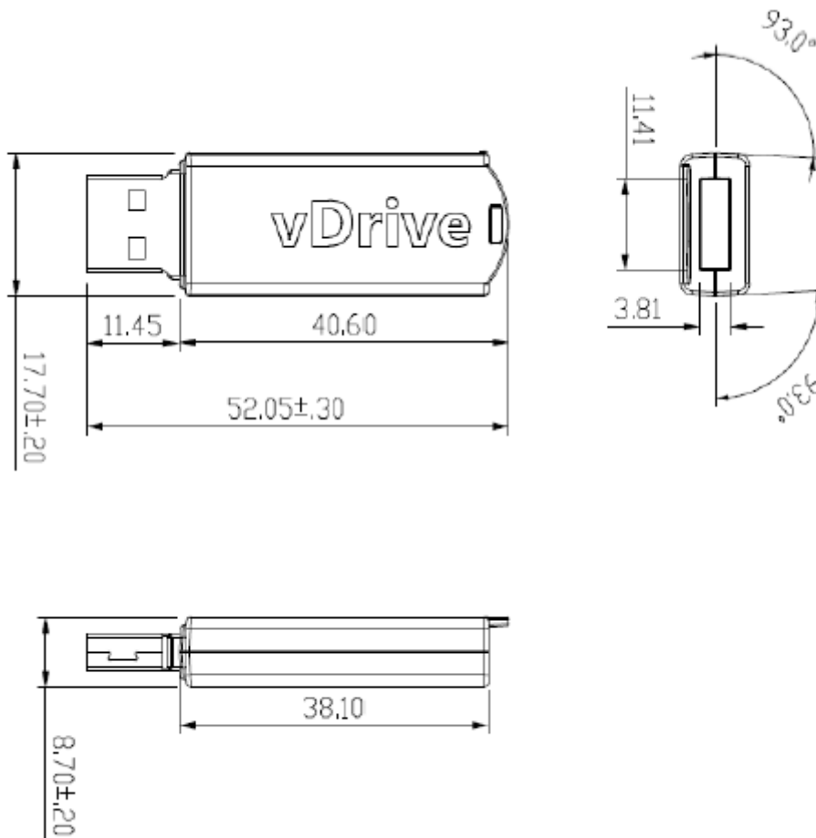
Figure 6-1 Dimensions
