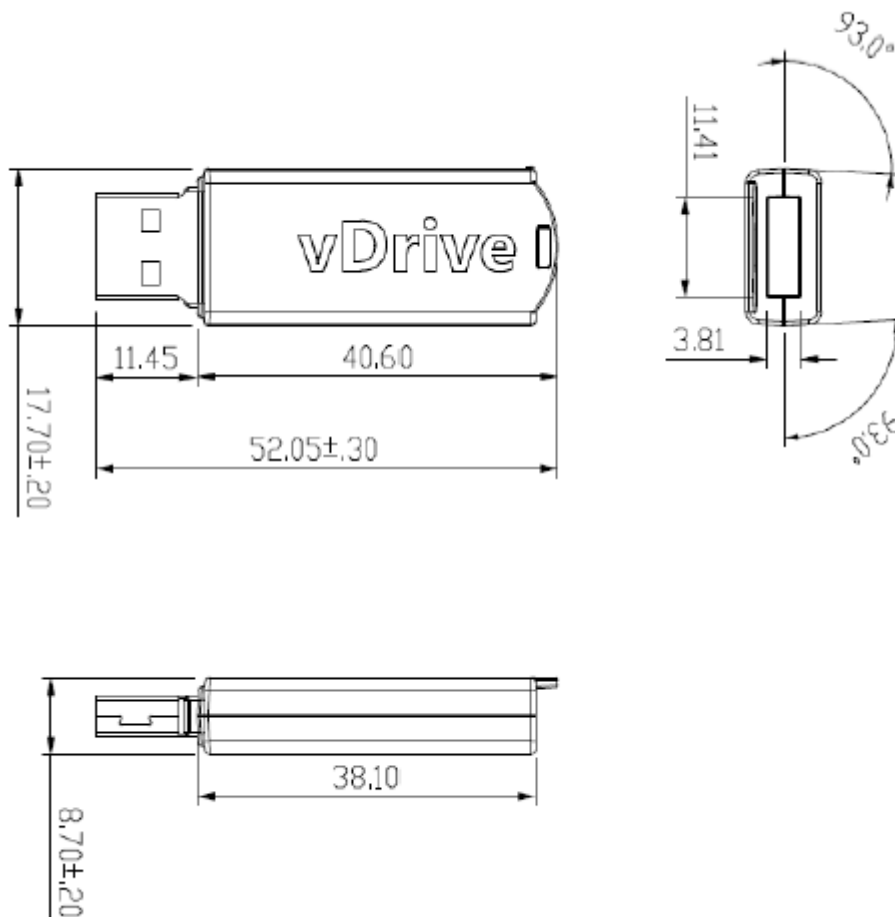
Figure 6-1 Physical Dimensions
