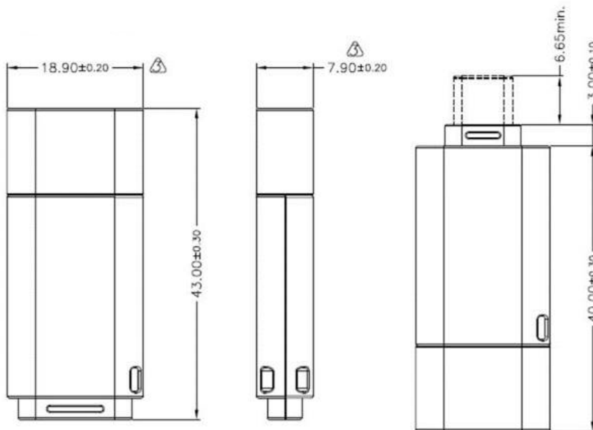
Figure 6-1 Physical Dimensions
