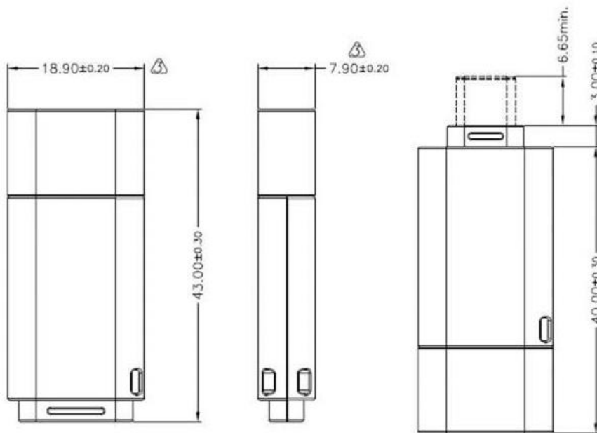
Figure 6-1 Physical Dimensions
