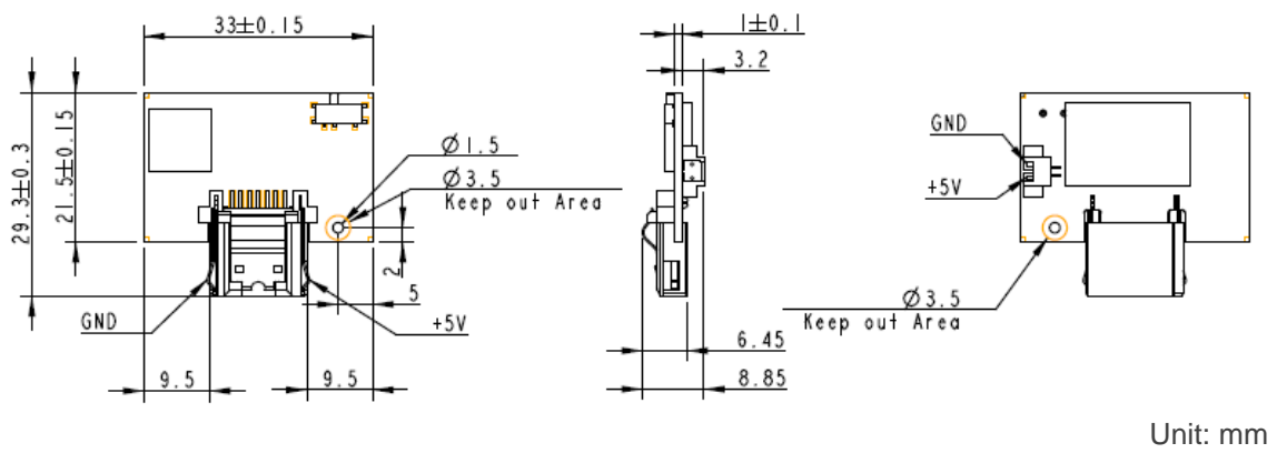
Figure 9-1 Physical Dimensions
