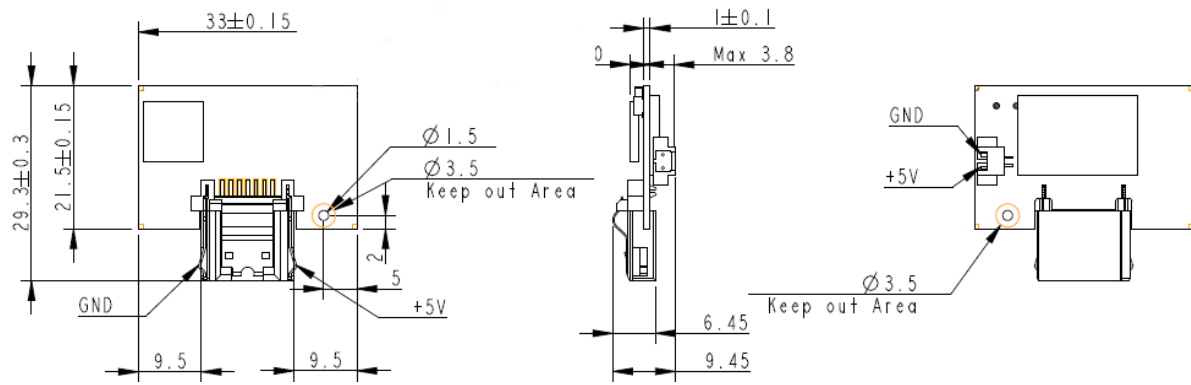
Figure 9-1 Physical Dimensions
