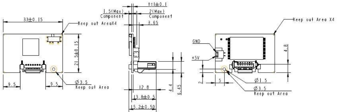
Figure 9-1 Physical Dimensions
