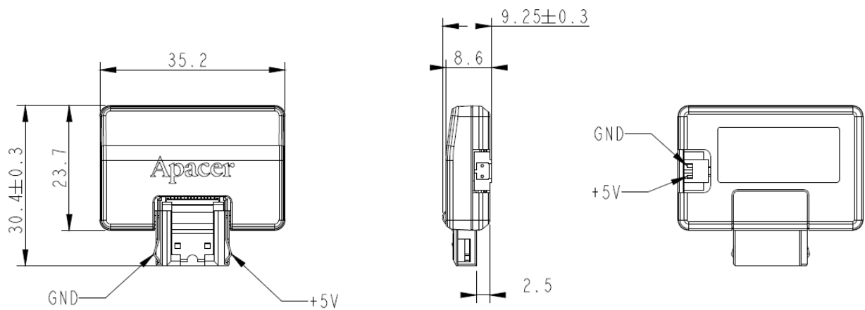
Figure 9-2 Dimensions – With Housing
