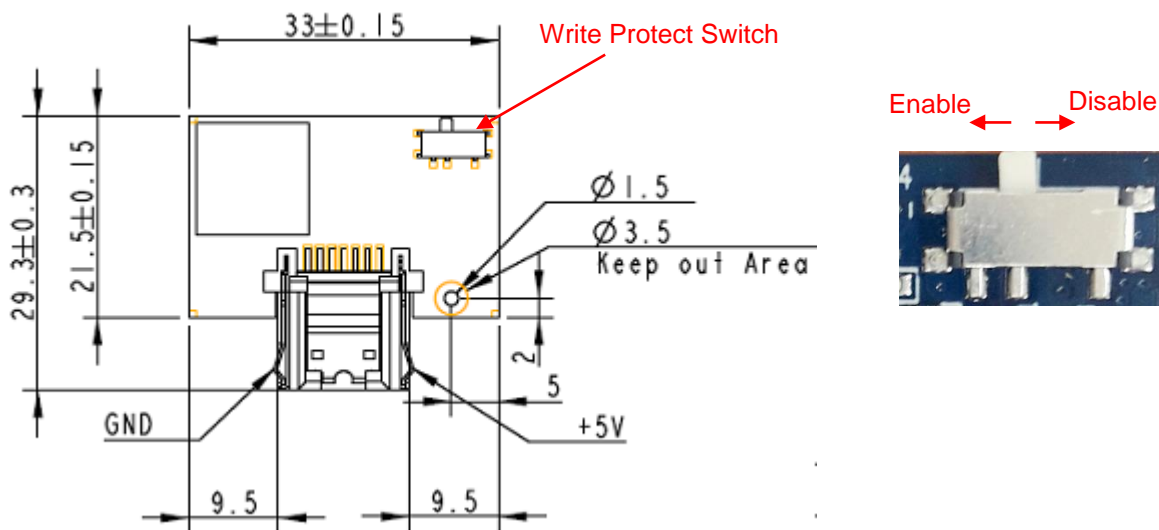
Figure 9-3 Write Protect Switch
