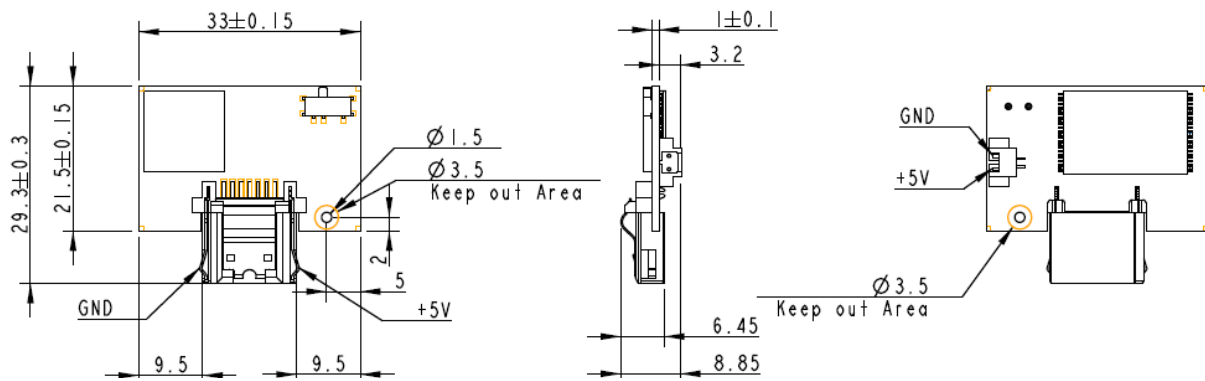
Figure 9-1 Dimensions – Without Housing
