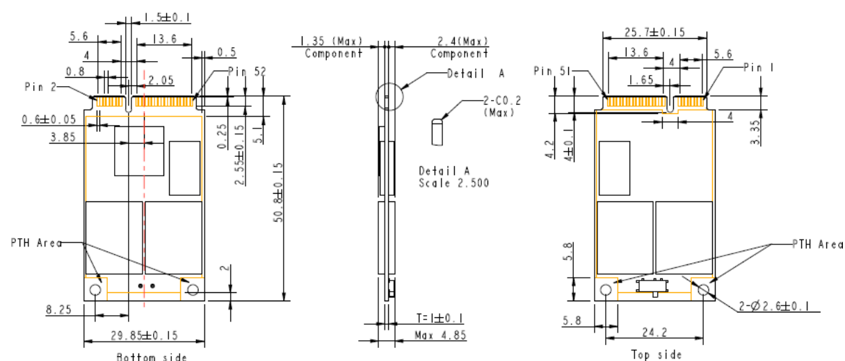
Figure 9-1 Physical Dimensions
