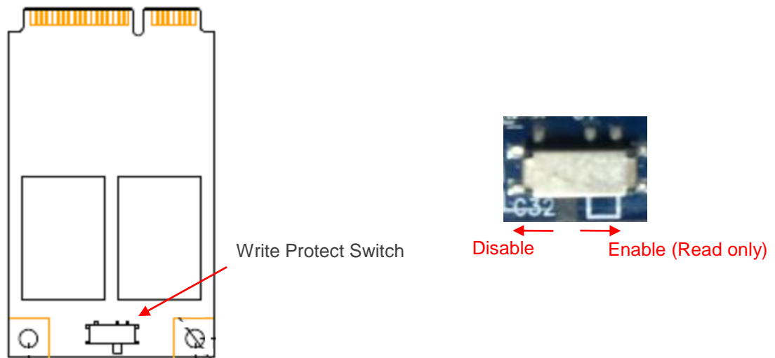
Figure 7-2 Write Protect Switch
