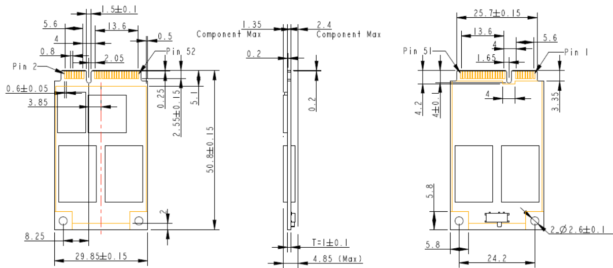
Figure 7-1 Dimensions
