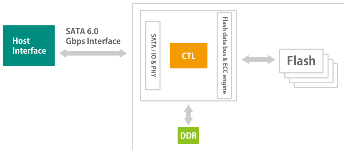
Figure 2-1 Block Diagram
