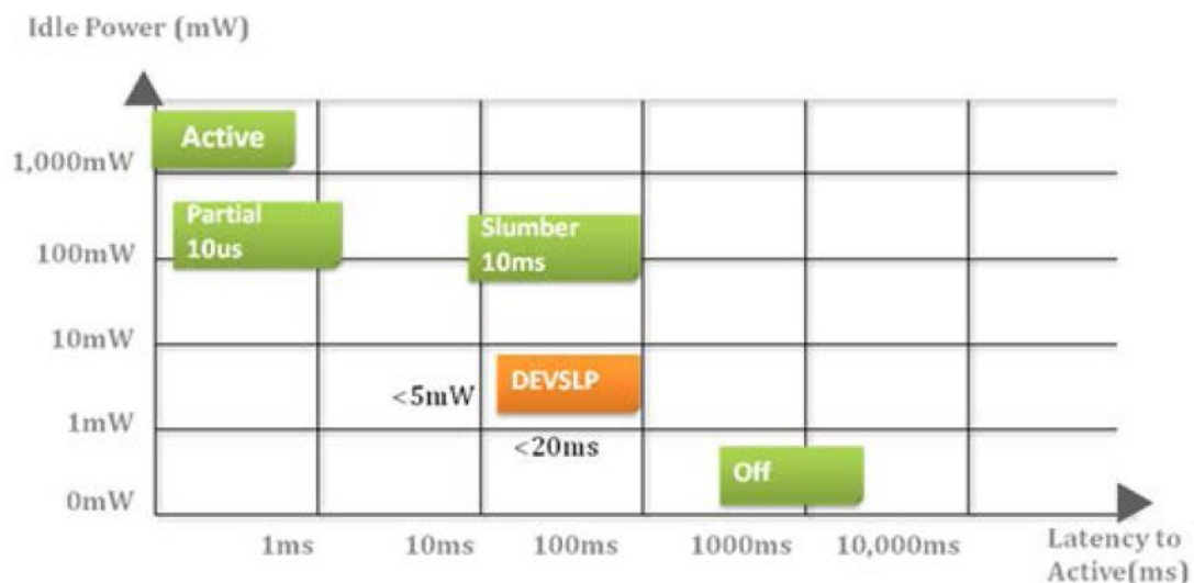
Figure 5-1 Device Sleep
