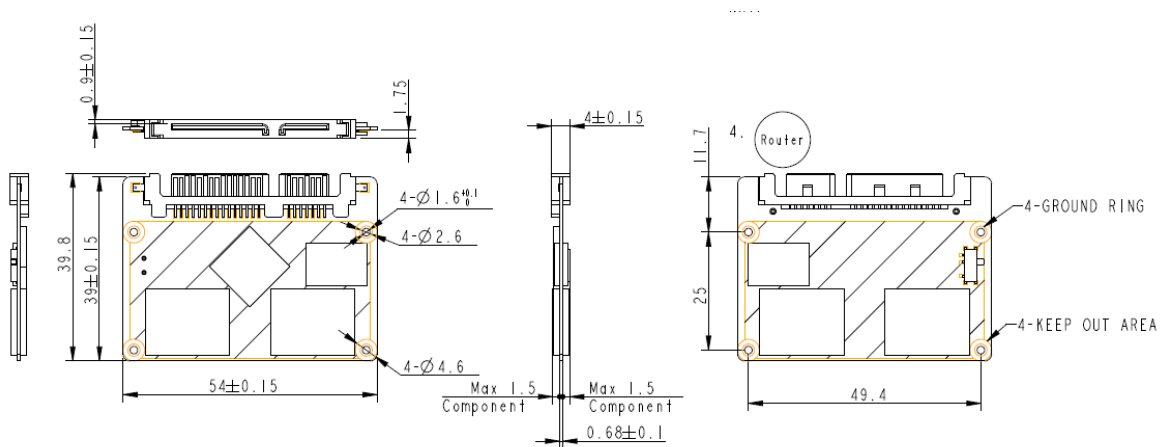
Figure 9-1 Physical Dimensions
