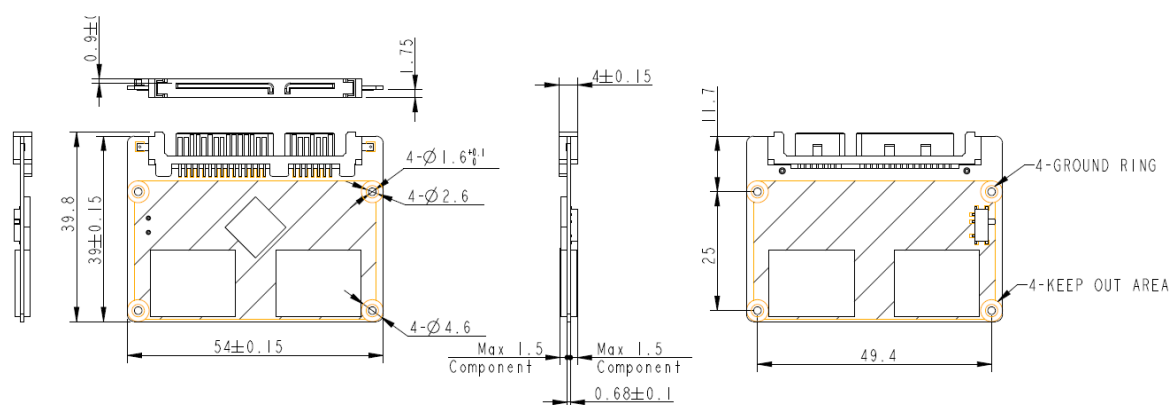
Figure 9-1 Physical Dimensions
