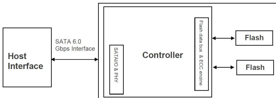
Figure 2-1 Block Diagram
