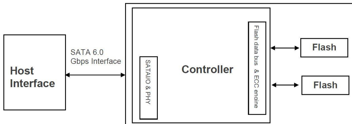
Figure 2-1 Block Diagram
