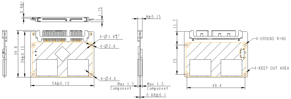
Figure 9-1 Physical Dimensions
