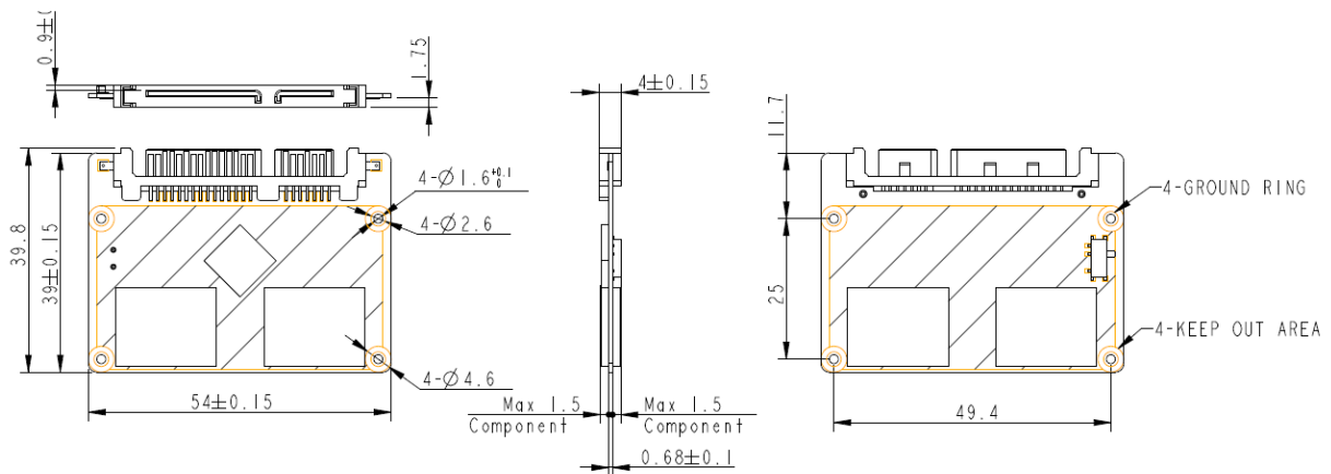
Figure 9-1 Physical Dimensions
