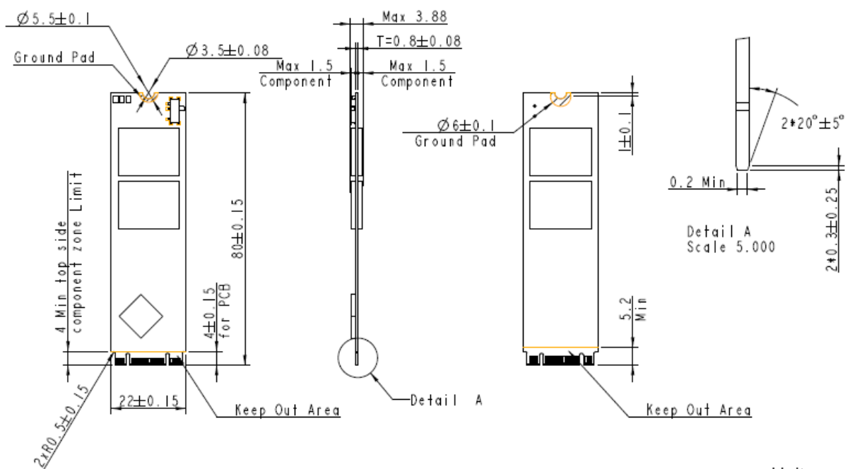
Figure 10-3 BGA Dimensions – Double Side
