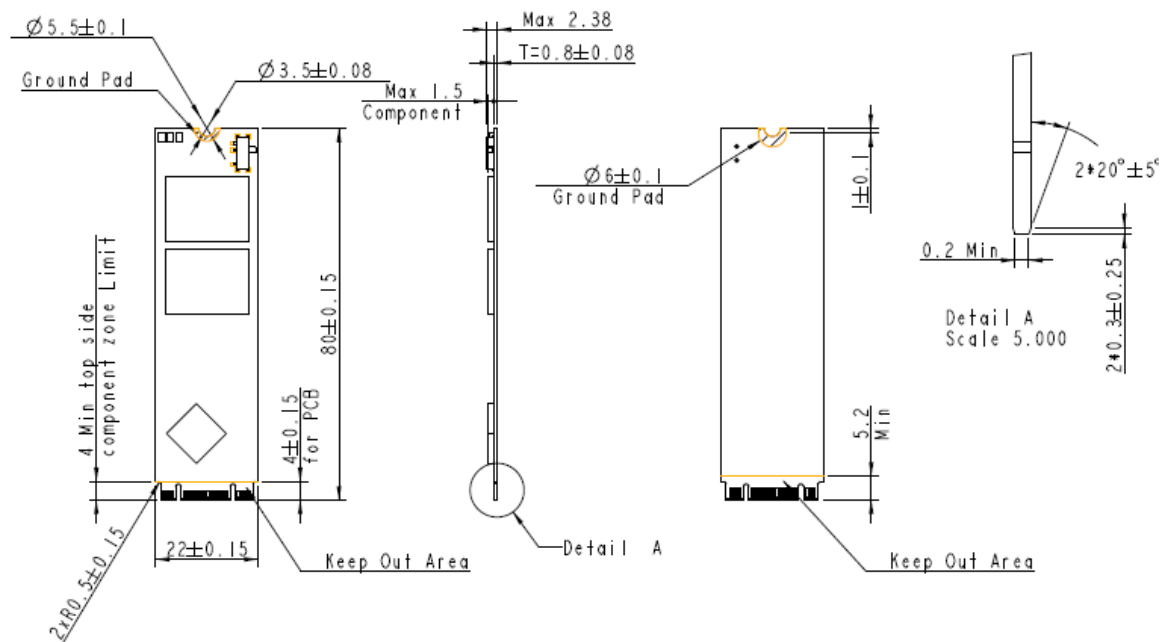
Figure 9-1 Single-side Dimensions
