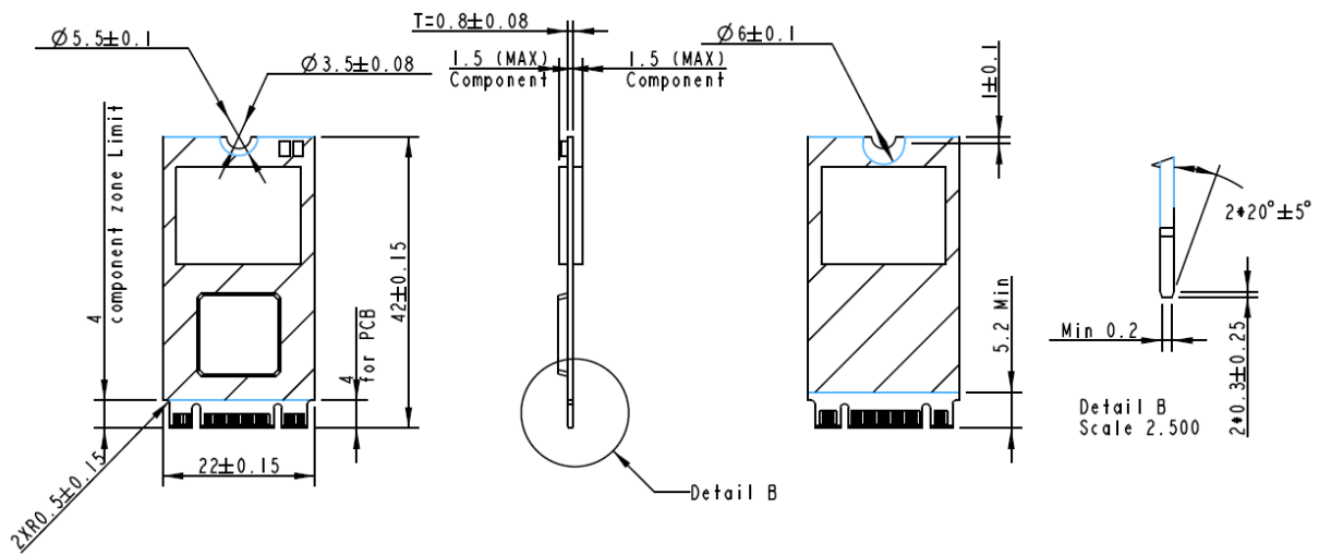
Figure 9-1 Physical Dimensions
