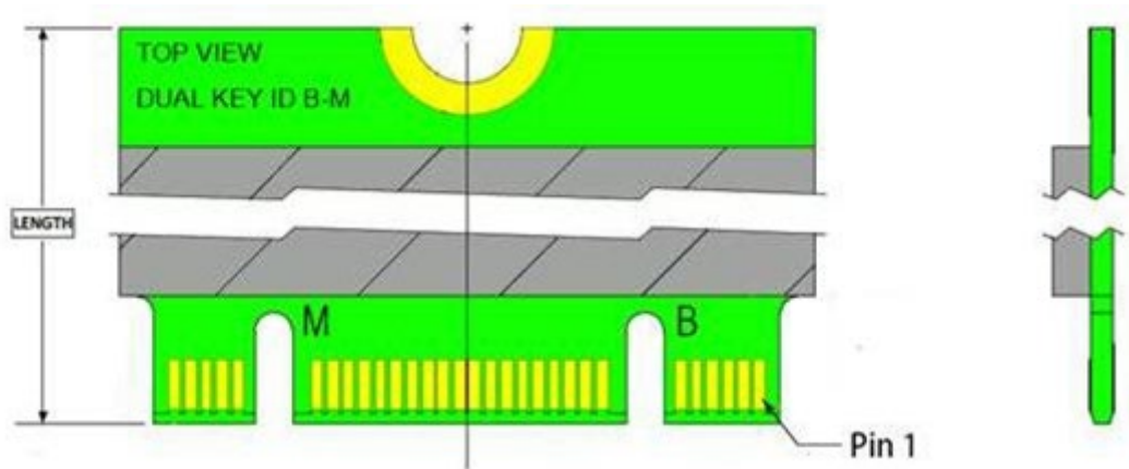
Figure 3-1 SATA Connectors
