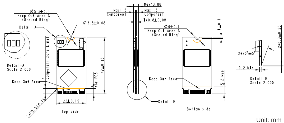
Figure 9-1 Physical Dimensions
