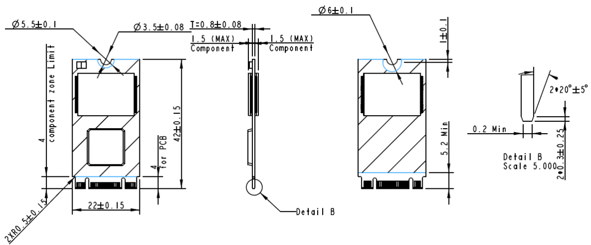
Figure 9-1 Physical Dimensions
