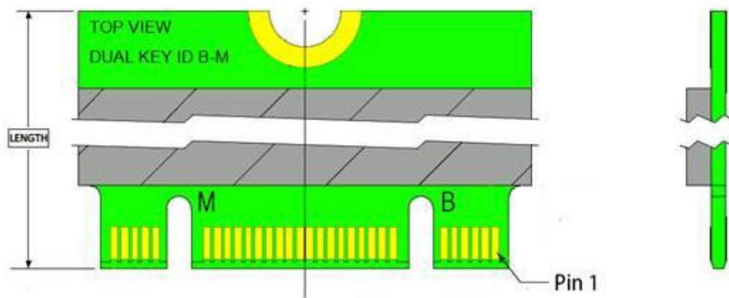
Figure 3-1 Pin Connectors
