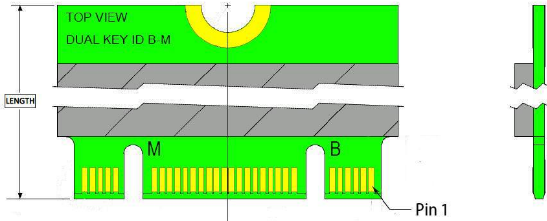
Figure 3-1 SATA Connectors
