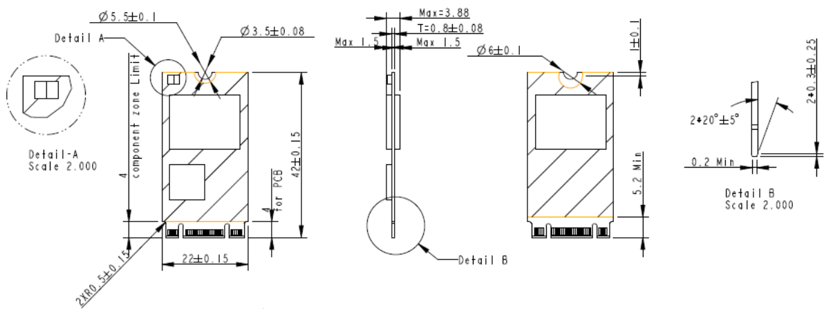
Figure 9-2 Dimensions – BGA
