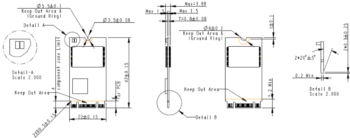
Figure 9-1 Dimensions – TSOP
