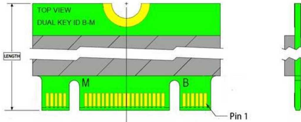
Figure 3-1 SATA Connectors
