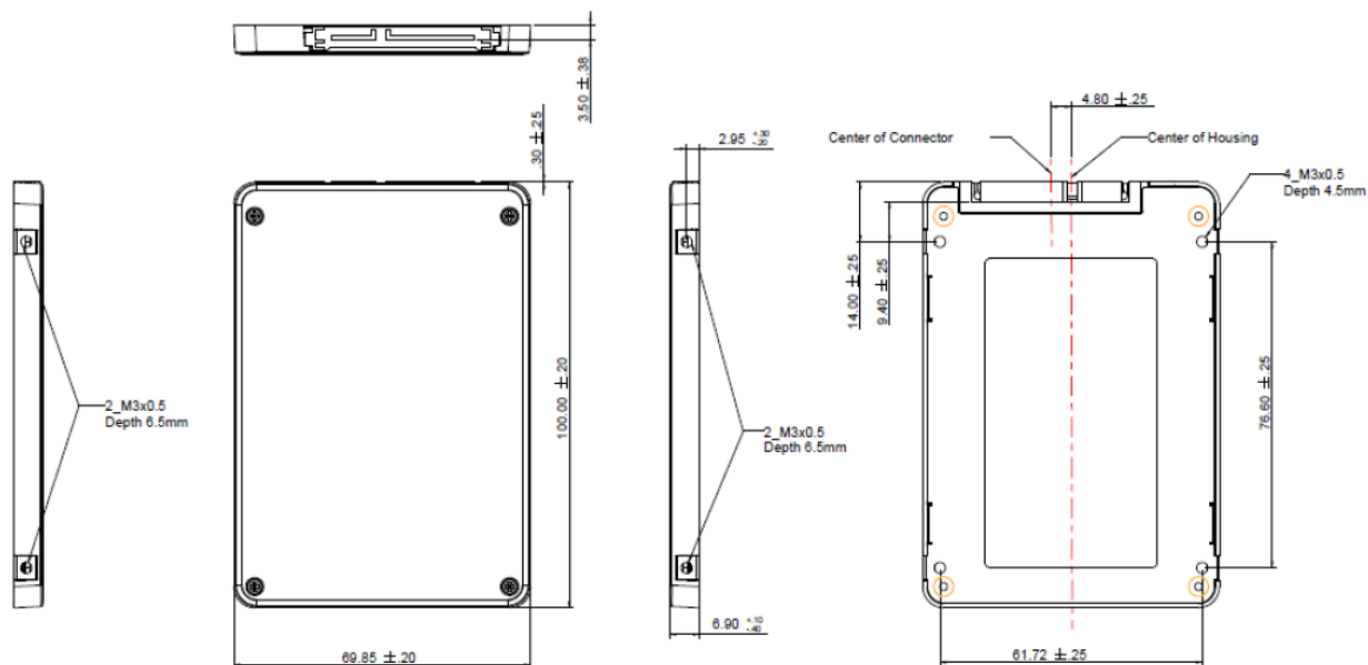
Figure 10-1 Physical Dimensions
