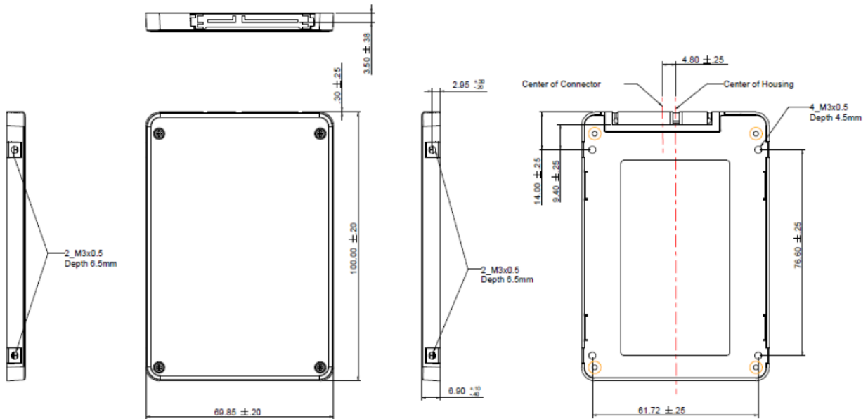
Figure 9-1 Physical Dimensions
