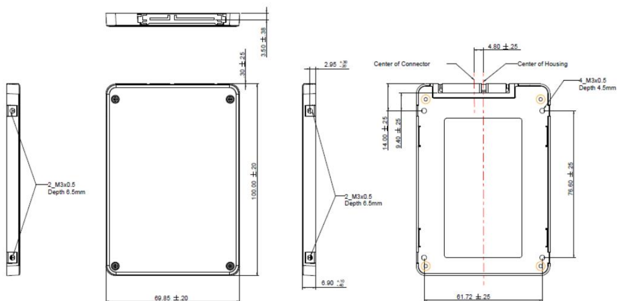
Figure 9-1 Physical Dimensions
