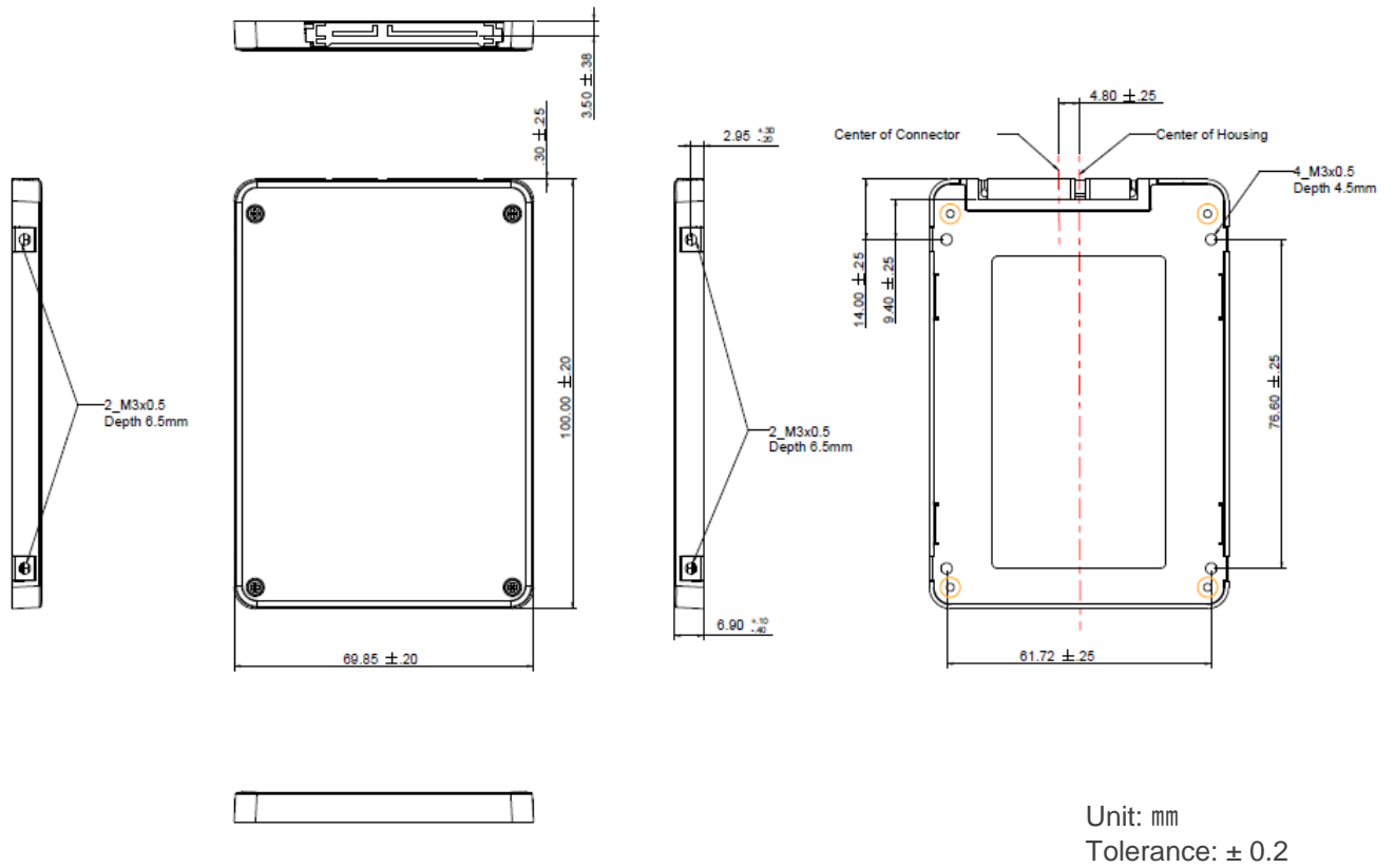
Figure 7-1 7mm Housing Physical Dimensions
