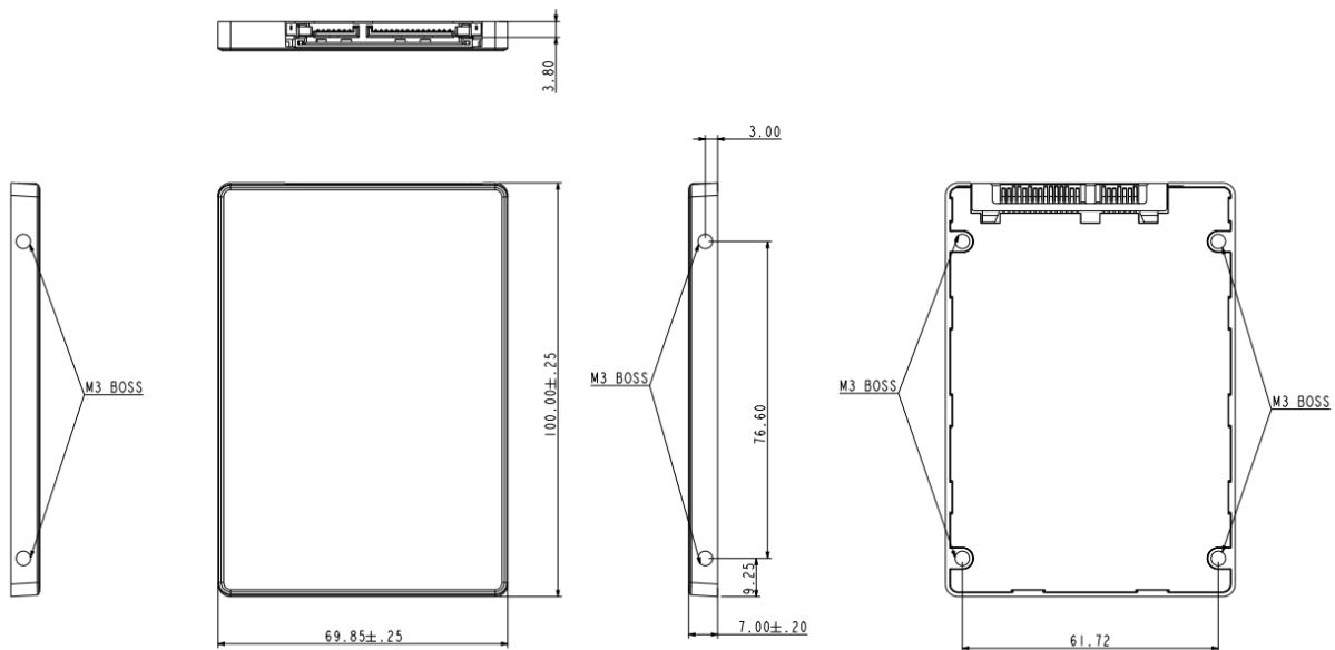
Figure 9-1 Physical Dimensions
