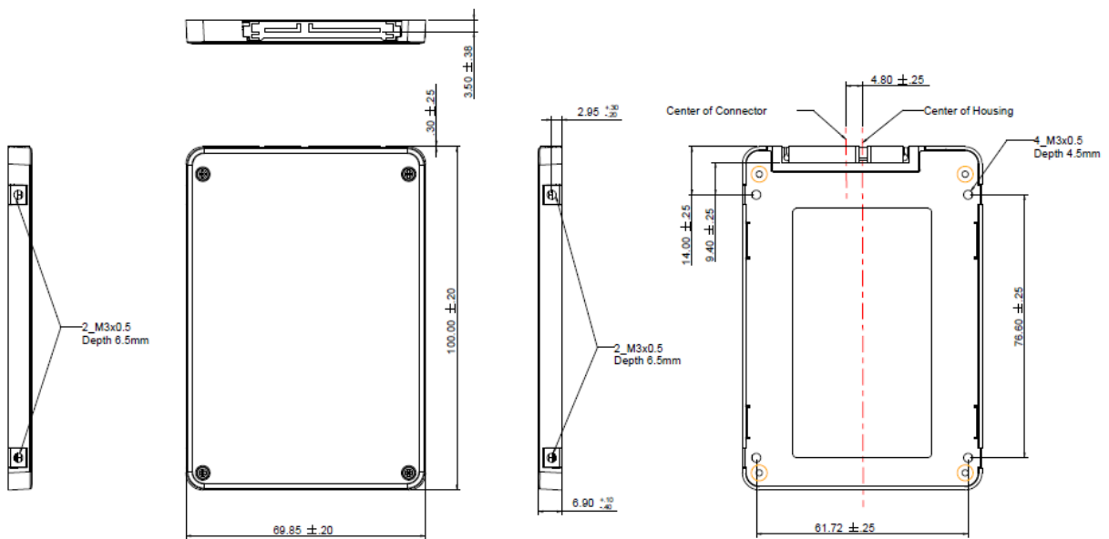
Figure 9-1 Physical Dimensions
