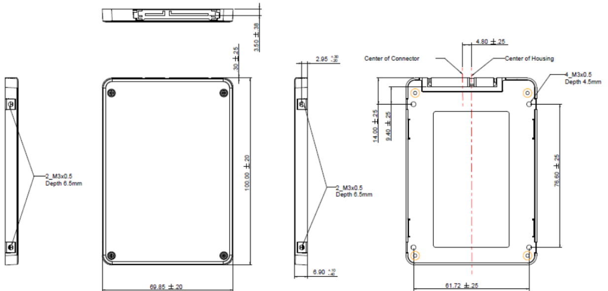
Figure 9-1 Physical Dimensions
