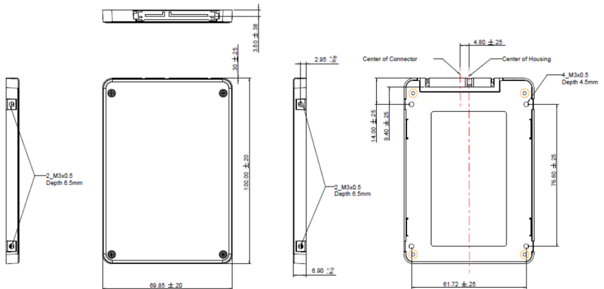
Figure 9-1 Physical Dimensions
