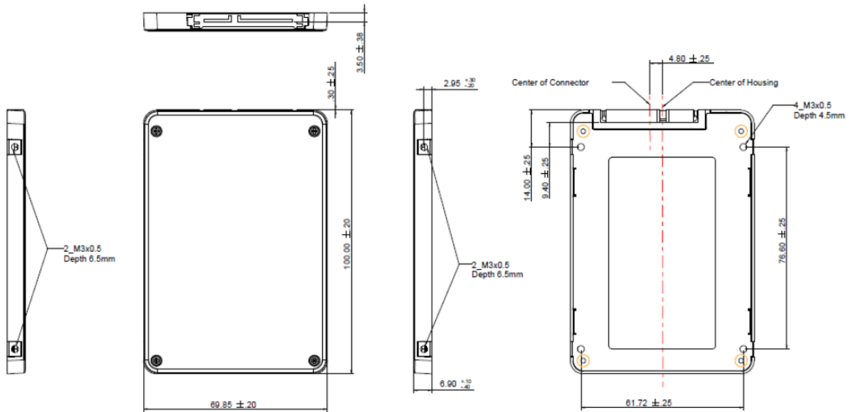
Figure 7-1 Physical Dimensions
