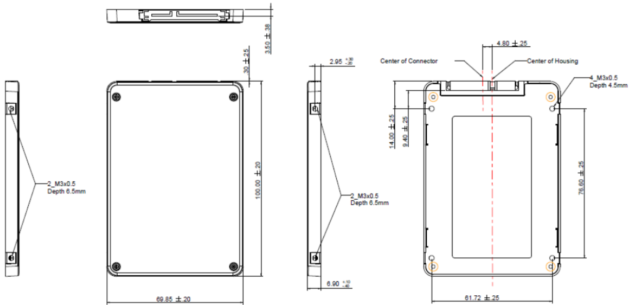
Figure 7-1 Physical Dimensions
