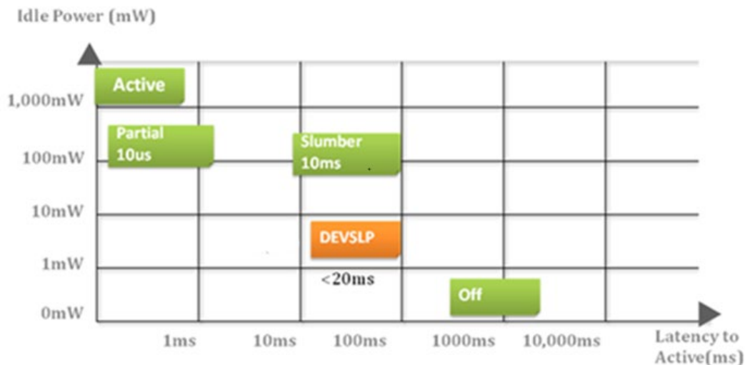
Figure 5-1 Device Sleep
