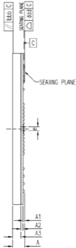
Figure 9-3 Dimensions – Side View
