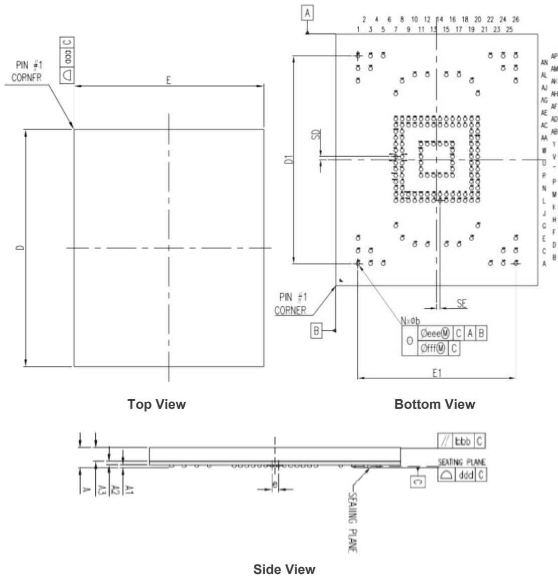
Figure 9-1 Physical Dimensions
