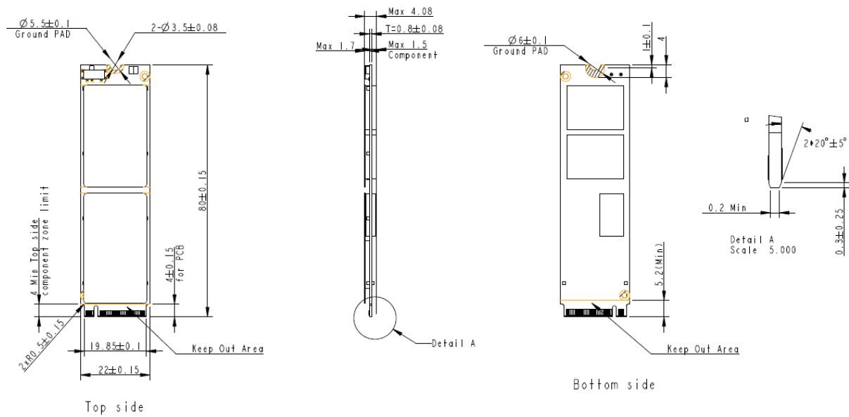
Figure 9-1 Dimensions
