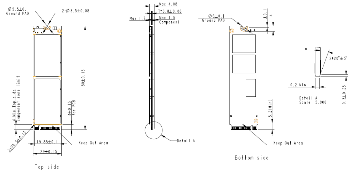
Figure 9-1 Dimensions
