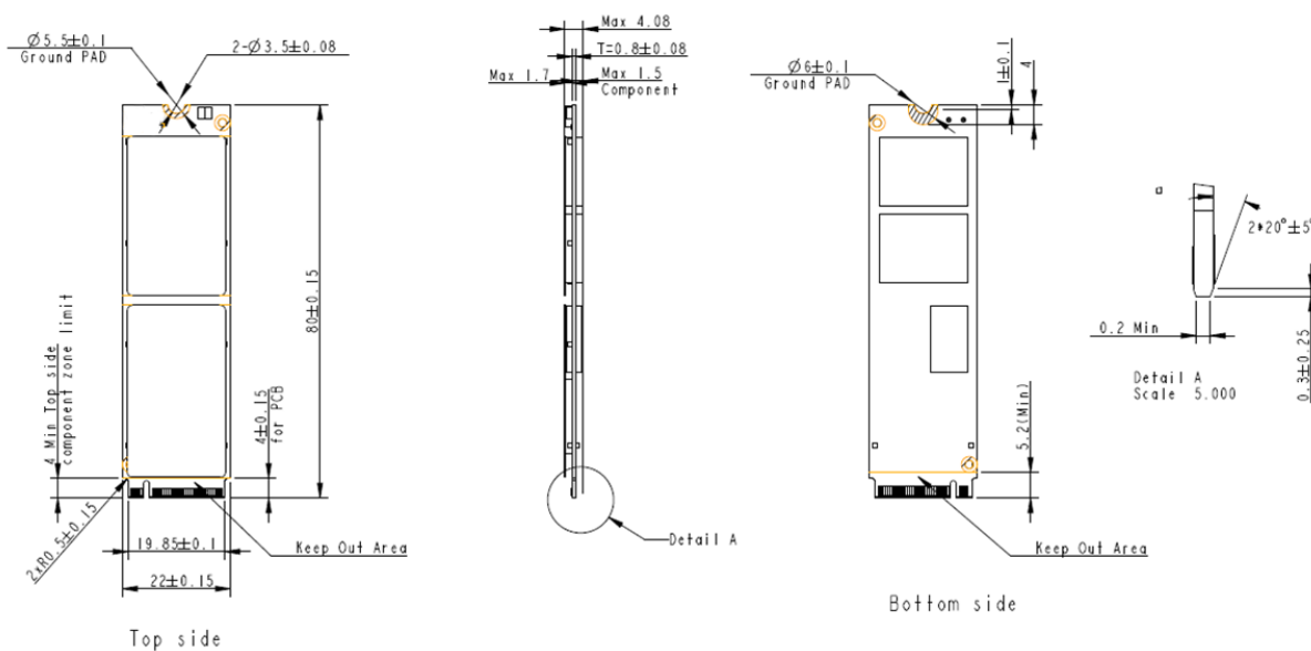
Figure 9-1 Physical Dimensions
