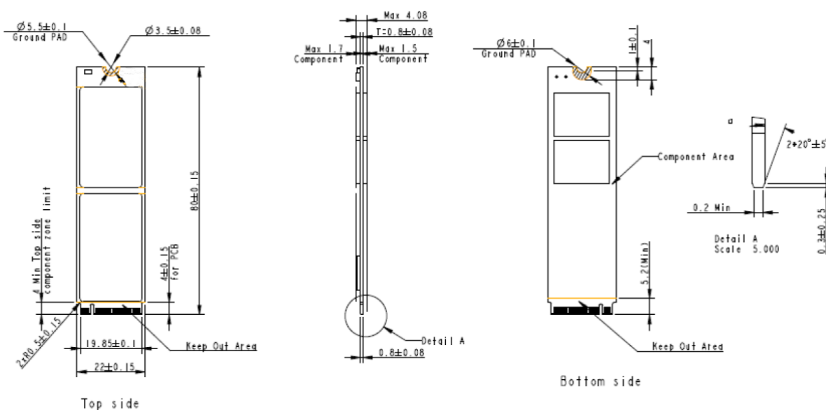
Figure 10-2 Double-sided Dimensions
