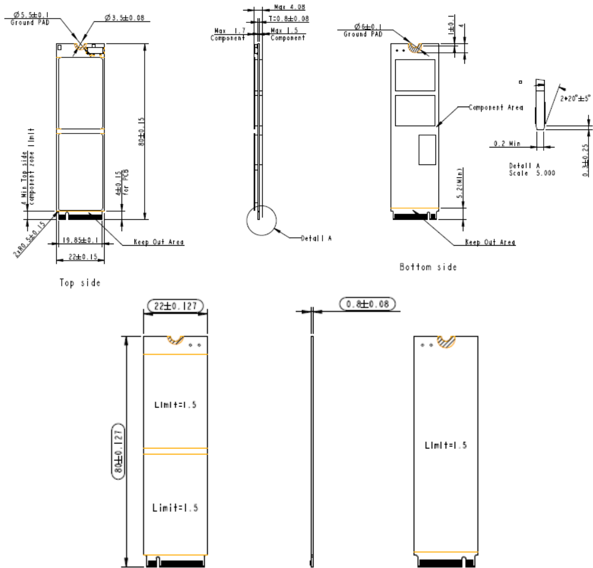
Figure 9-2 Dimensions – CoreGlacier
