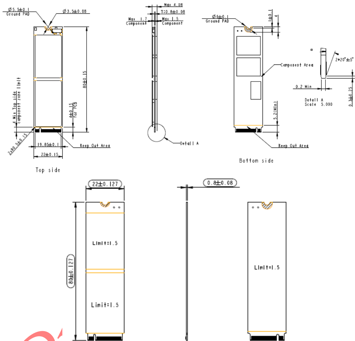
Figure 9-2 Dimensions – CoreGlacier
