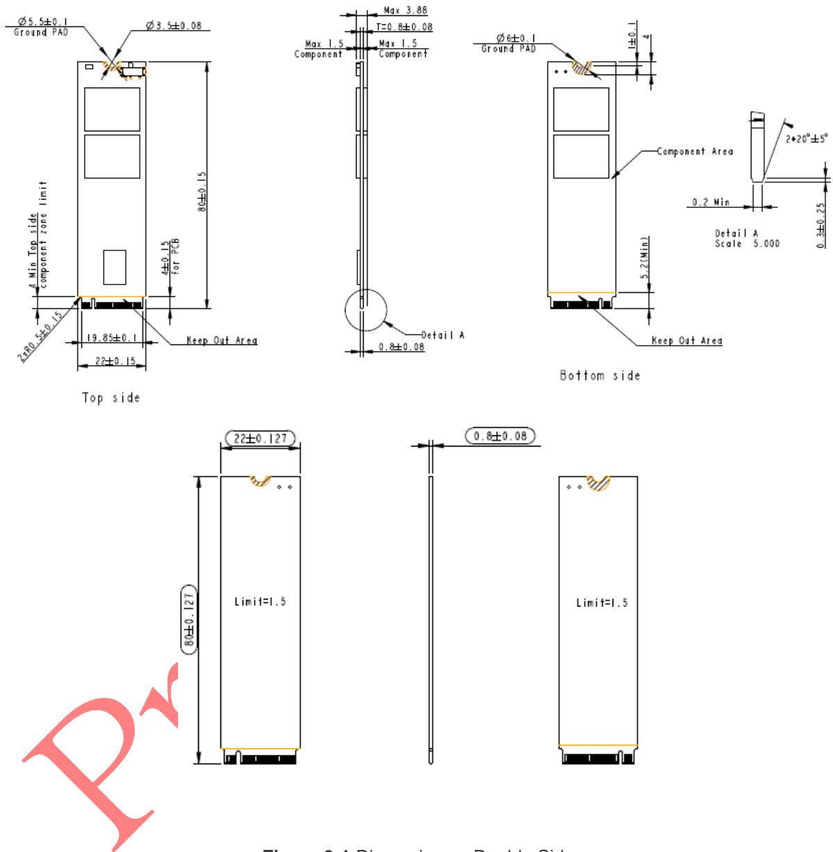
Figure 9-1 Dimensions – Double Side
