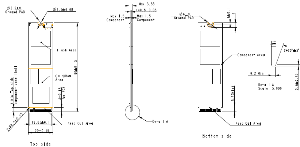
Figure 9-1 Double-sided Dimensions
