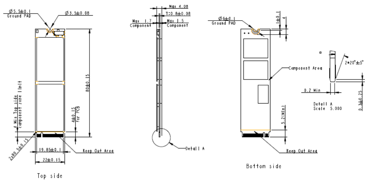
Figure 9-2 CoreGlacier Dimensions
