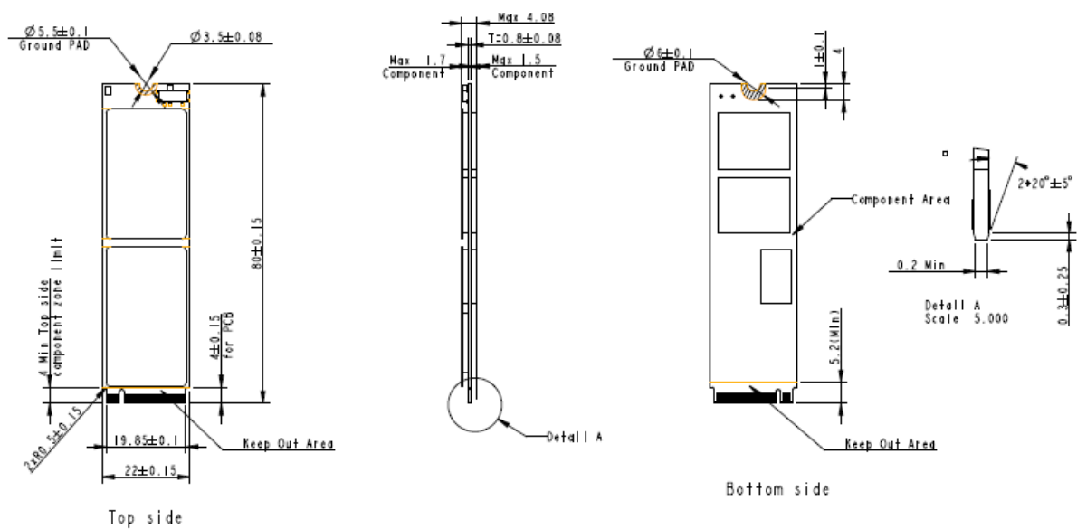
Figure 9-2 Dimensions – CoreGlacier
