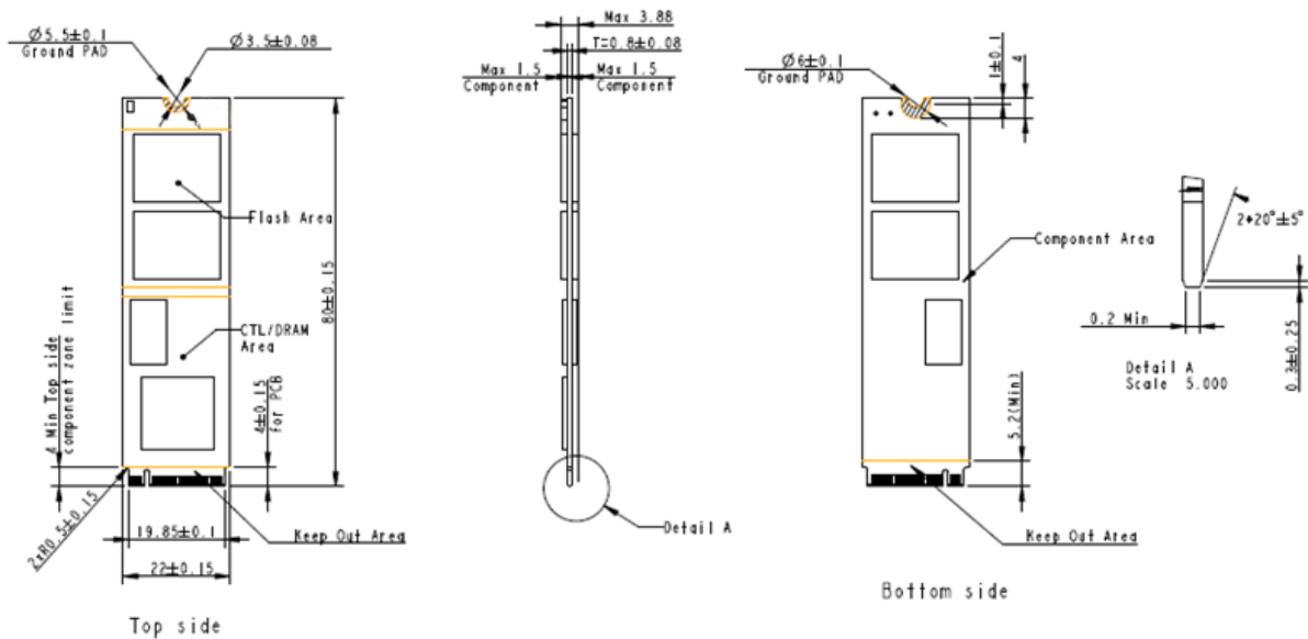
Figure 9-1 Double-sided Dimensions
