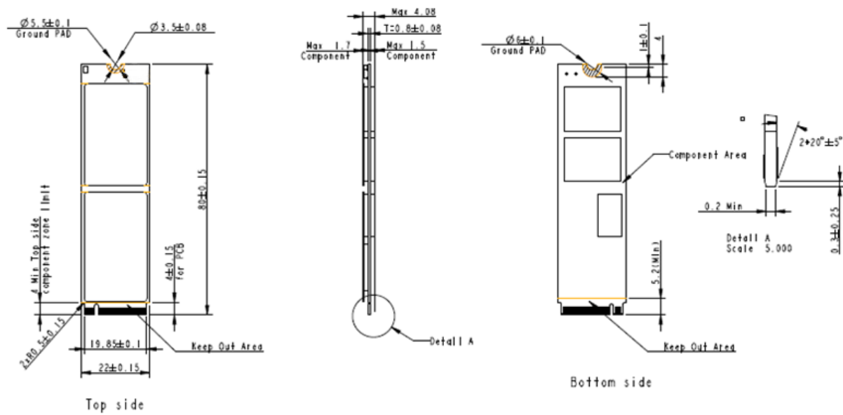
Figure 9-2 CoreGlacier Dimensions
