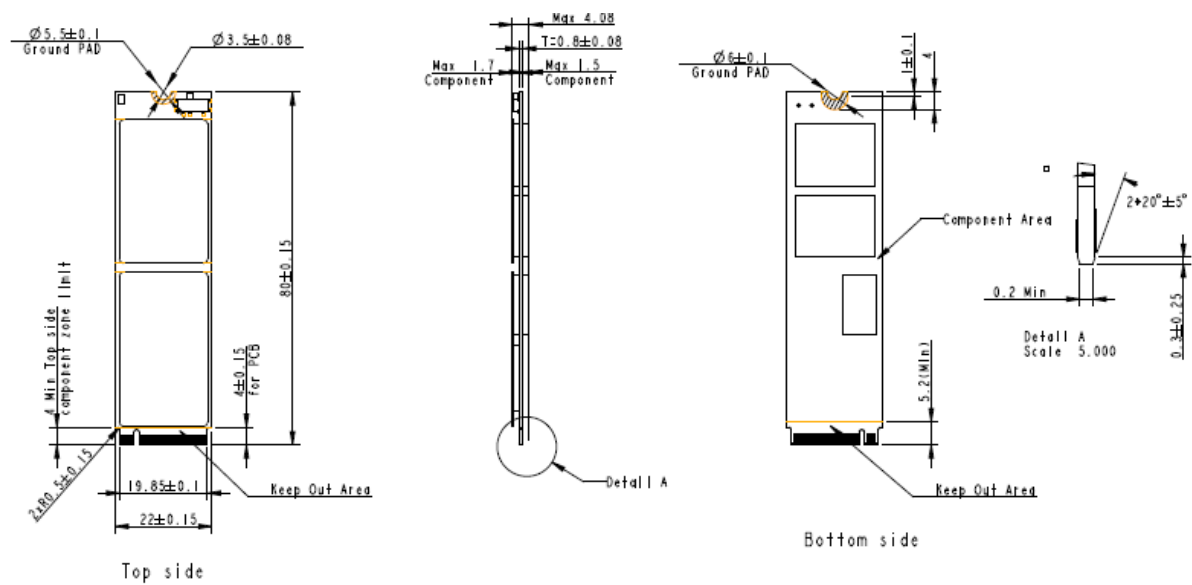
Figure 9-2 CoreGlacier Dimensions
