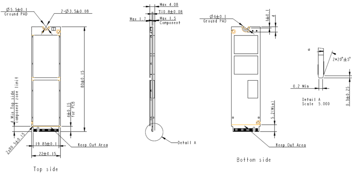
Figure 9-1 Physical Dimensions
